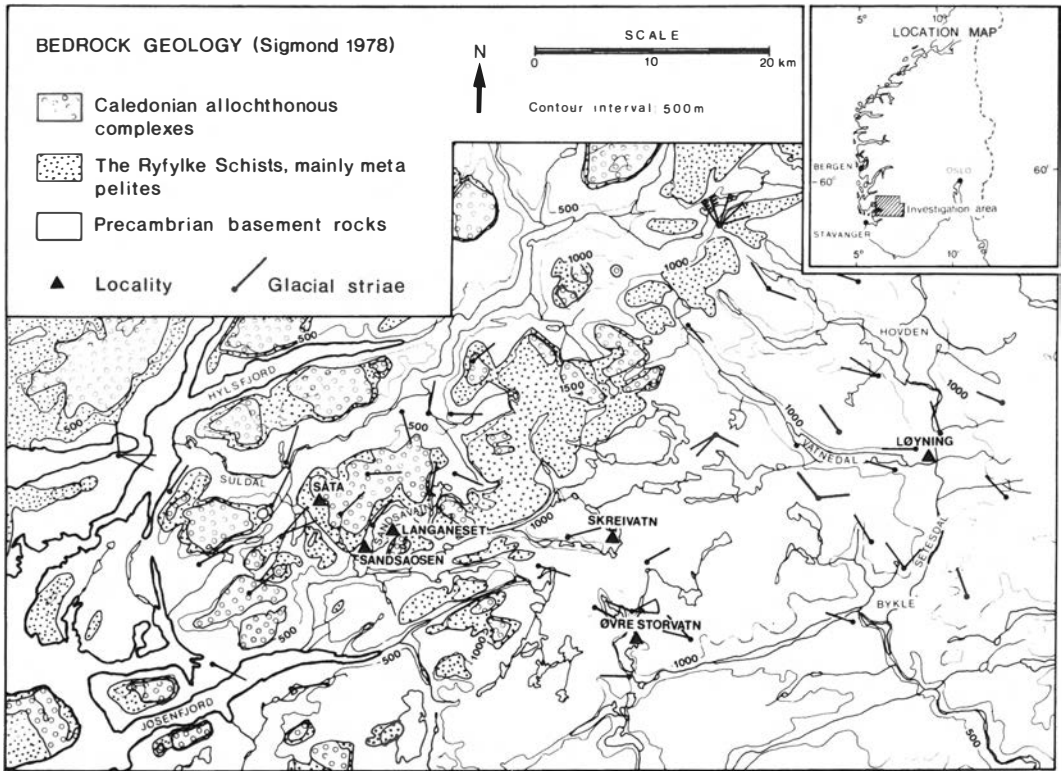
Fig. 1. Map showing the location of the six investigated localities, the bedrock geology (Sigmond 1978) and selected glacial striae (Anundsen (1972) for the western part and Blystad (1978) for the eastern part).
