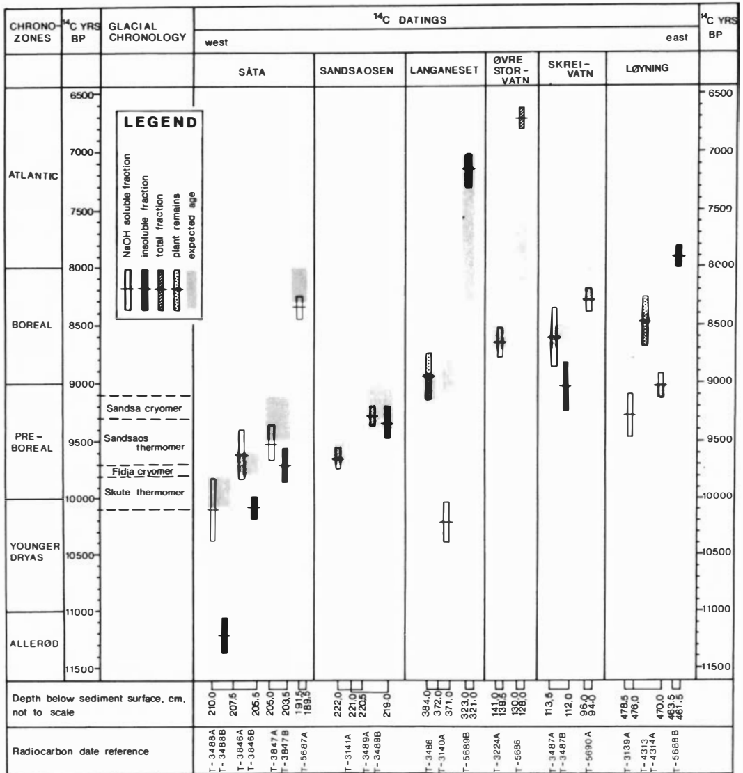
Fig. 2. Graphic representation of the radiocarbon dates with one standard deviation. The westernmost locality is presented to the left and the easternmost to the right. The radiocarbon dates at one locality are presented in stratigraphic order with the result of the lowest dated level to the left and the highest dated level to the right. The position is indicated on the horizontal scale. The expected age for each dating is shaded.
