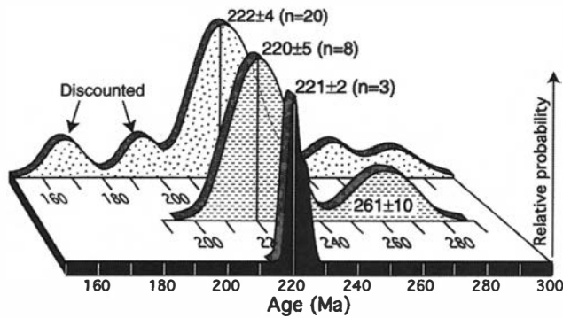
Fig. 2. Probability plot showing results of K-Ar and ^{40}\text{Ar}/^{39}\text{Ar} dating of dolerite dikes from Sunnhordland. Front: ^{40}\text{Ar}/^{39}\text{Ar} plateau ages of the three dikes re-dated in this study (Table 1). Middle: Amphibole K-Ar ages from 5 dikes, recalculated from Færseth et al. (1976). Back: Whole-rock ages from 15 dikes, recalculated from Færseth et al. (1976). The three data sets consistently show very distinct peaks at about 220 Ma. In addition, two amphibole dates from one of the dikes show a \sim 260 Ma age, giving rise to the additional peak in the central graph. The two Jurassic whole-rock ages are discarded as ages of intrusion because of alteration (see text for discussion). All errors involved in the calculation of the plots were 2\sigma . Weighted mean and 2 s.d. errors of Triassic probability peaks are shown.
