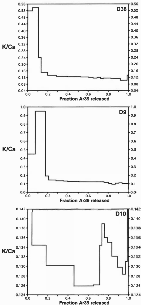
Fig. 5. K/Ca distribution for the amphibole separates analyzed by the ^{40}\text{Ar}/^{39}\text{Ar} method. See text for discussion.
