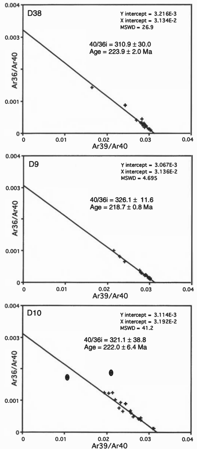
Fig. 6. Inverse isochron plot of ^{40}\text{Ar}/^{39}\text{Ar} data from the three dikes dated in this study. The isochron ages are indistinguishable from the plateau ages presented in Fig. 4. Two data points were disregarded for dike D10; the gas associated with these two deleted steps is largely unradiogenic and is adversely affected by system blanks, thus they are not useful in calculating the isochron age.
