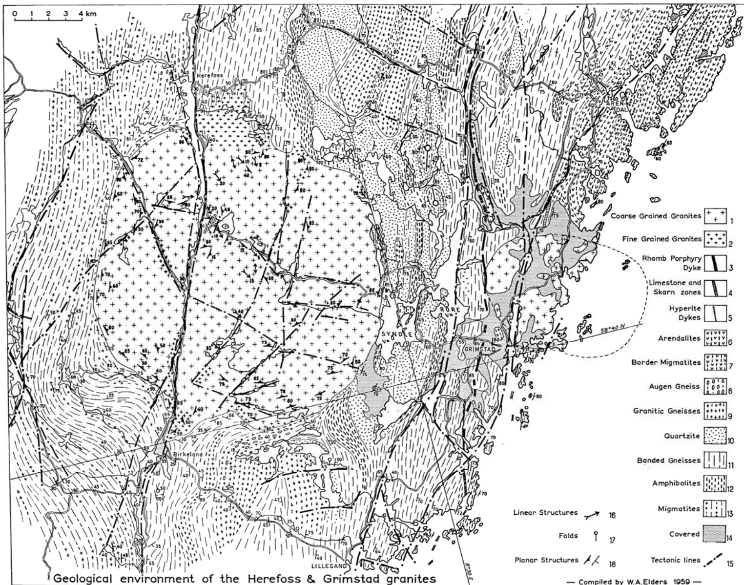
Fig. 1. Geological environment of the Herefoss and Grimstad granites.
